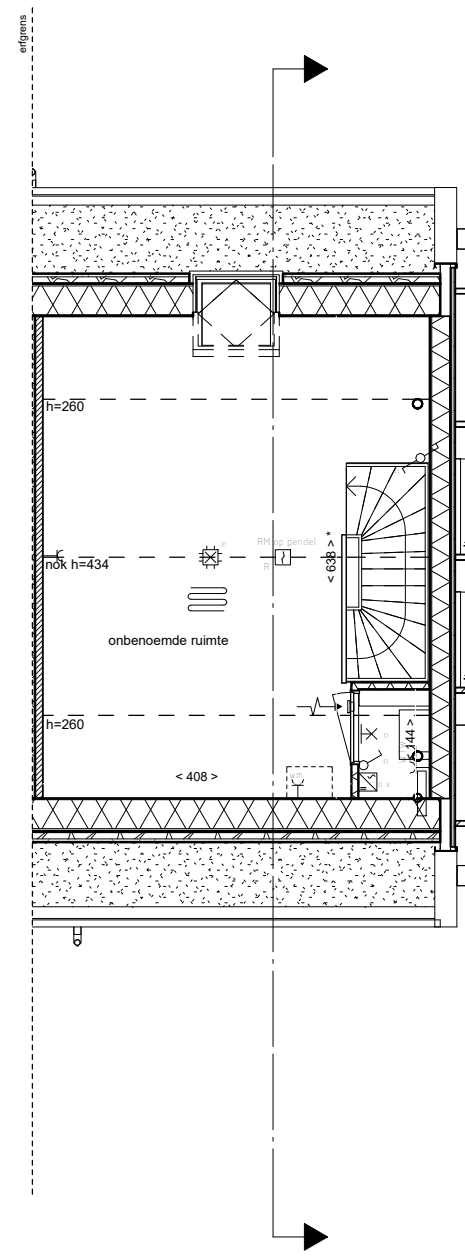
zolder
