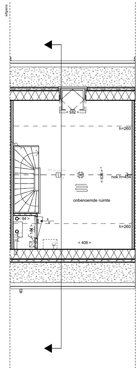
zolder
