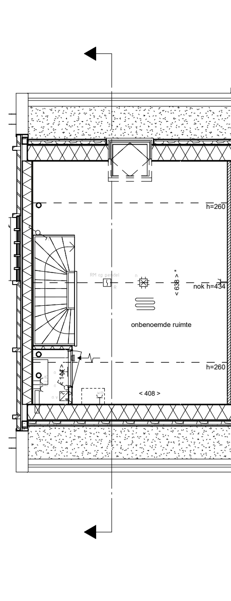
zolder
